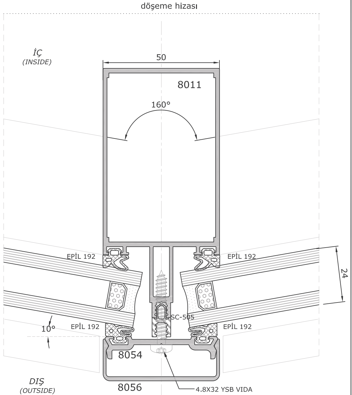
Detay Detail 4
